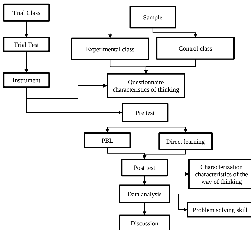
Figure 1. Research Flowchart
